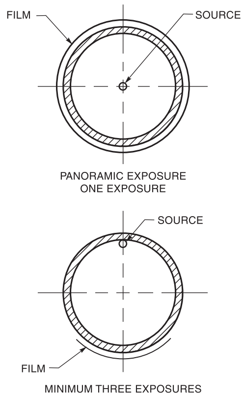
Figure 9.31—Single-Wall Exposure— Single-Wall View (see 9.29.1.1)
