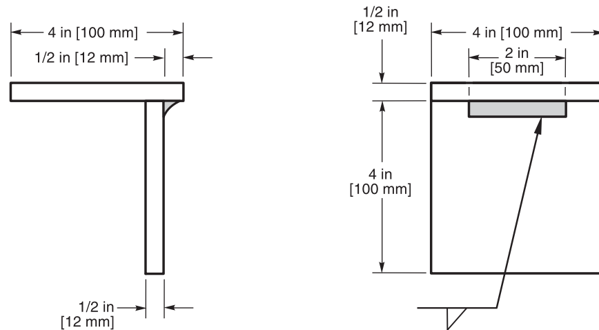
Figure 4.27—Fillet Weld Break Specimen—Tack Welder Qualification (see 4.16.2)
