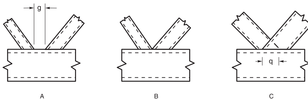
Figure C-9.5—Transition Between Gap and Overlap Connections (see C-9.6.2.1)
