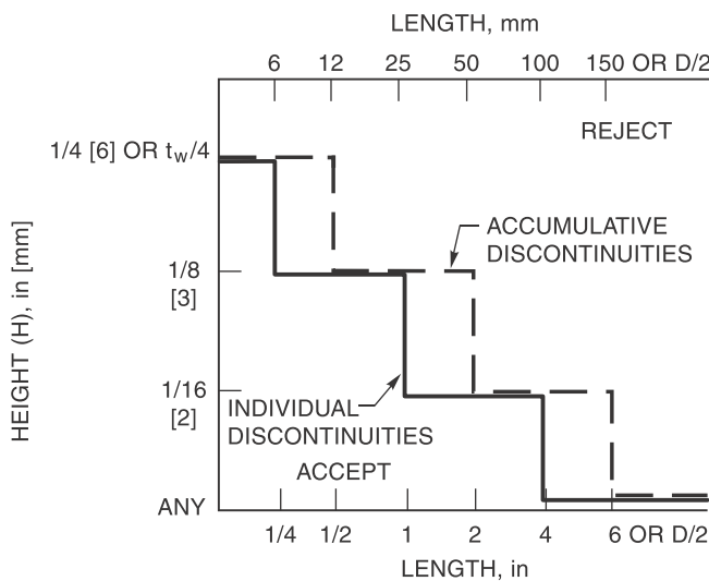
Figure 9.30—Class X Indications (see 9.27.1.2)
