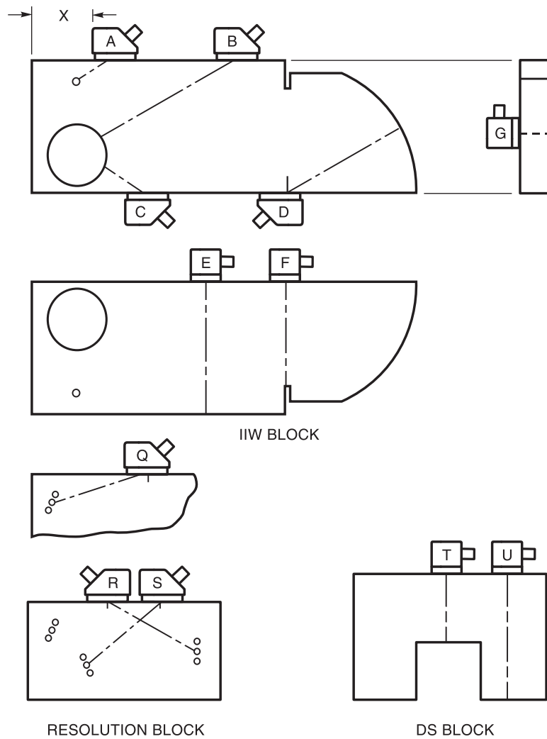
Figure 6.16—Transducer Positions (Typical) (see 6.22, 6.27, and 6.28)
