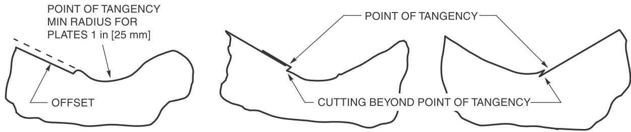
Figure C-5.1—Examples of Unacceptable Reentrant Corners (see C-5.15)
