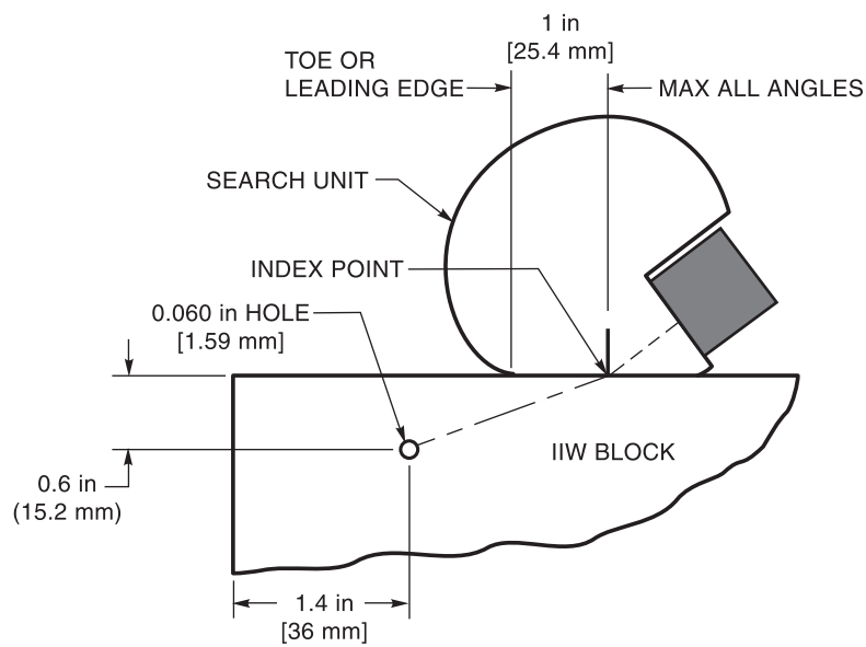
Figure 6.12—Qualification Procedure of Search Unit Using IIW Reference Block (see 6.21.7.7)
