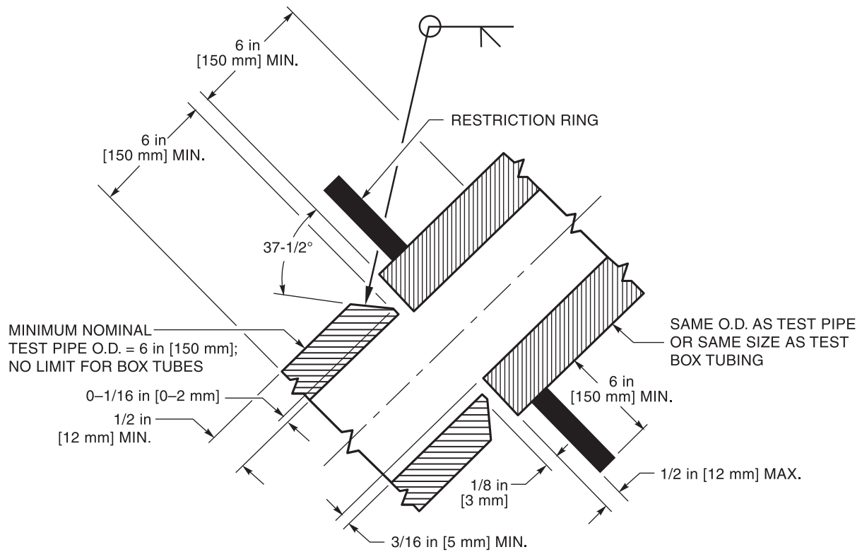
Figure 9.25—Test Joint for T-, Y-, and K-Connections without Backing on Pipe or Box Tubing ( \geq 6 in [150 mm] O.D.)—Welder and WPS Qualification (see 9.15.4.1 and 9.19)
