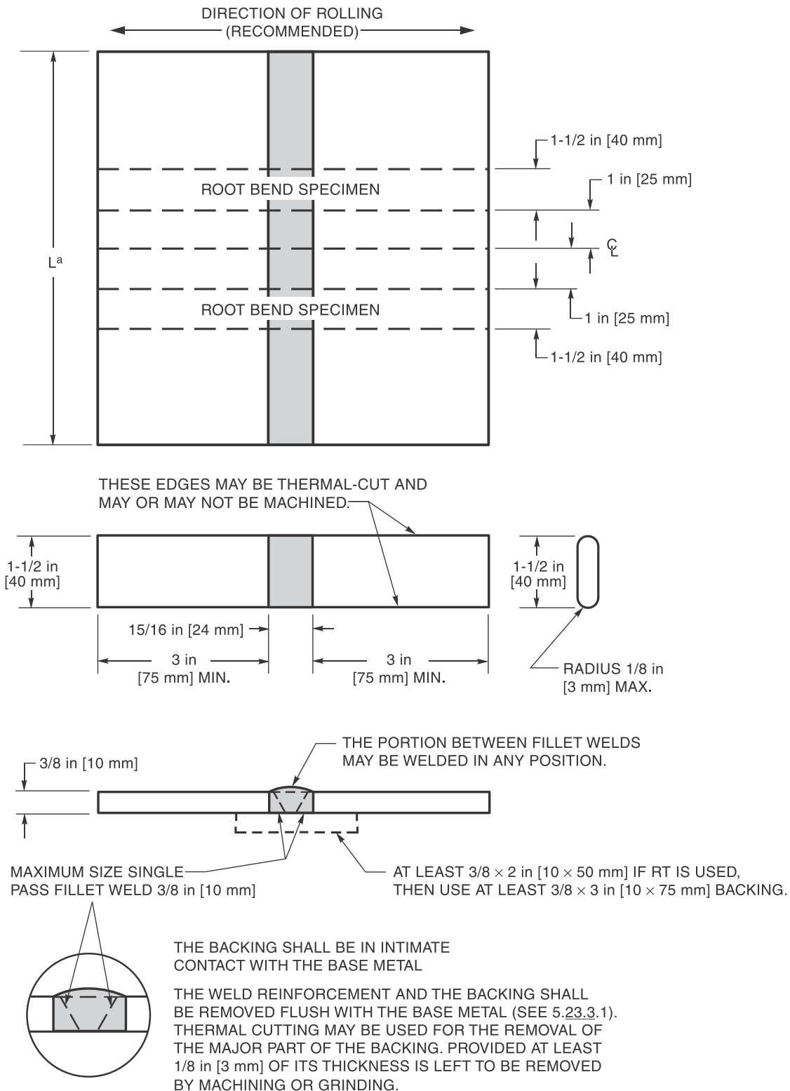
Figure 4.22—Fillet Weld Root Bend Test Plate—Welder or Welding Operator Qualification—Option 2 (see 4.21.2 and Table 4.11 or 9.21 and Table 9.14)
