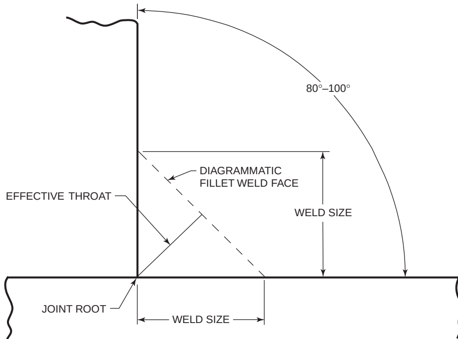
Figure A.1—Fillet Weld (see 2.4.2.6)
