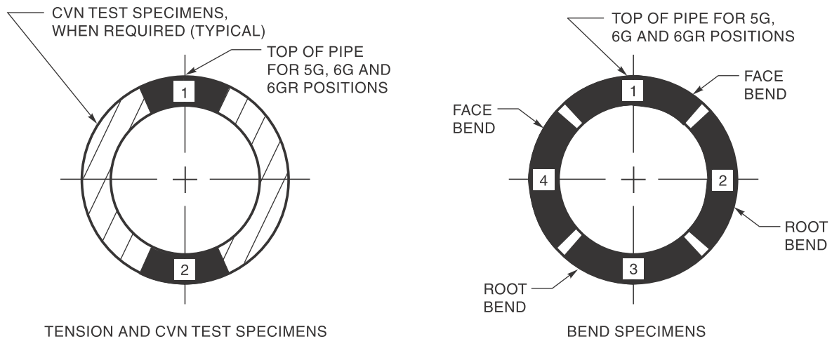
DETAIL A —2 in [50 mm] OR 3 in [75 mm] IN DIAMETER
