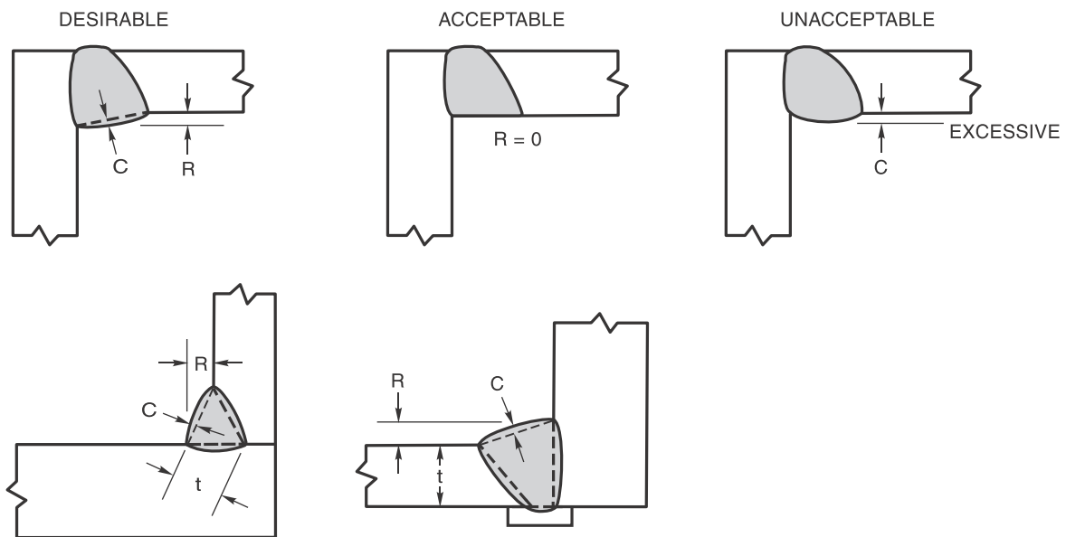
Figure 5.4—Requirements for Weld Profiles (see Tables 5.8 and 5.9)
