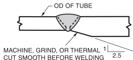
(D) TRANSITION BY TAPER BORE OF THICKER TUBE
