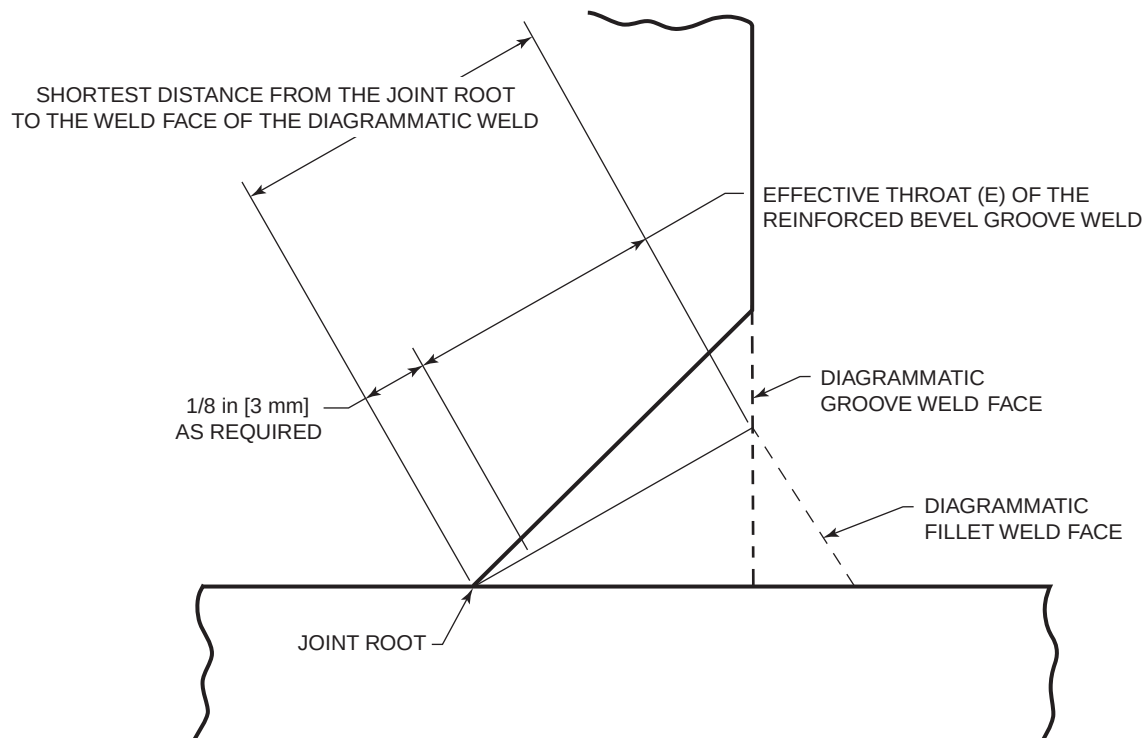
Figure A.3—Bevel Groove Weld with Reinforcing Fillet Weld (see 2.4.2.7)
