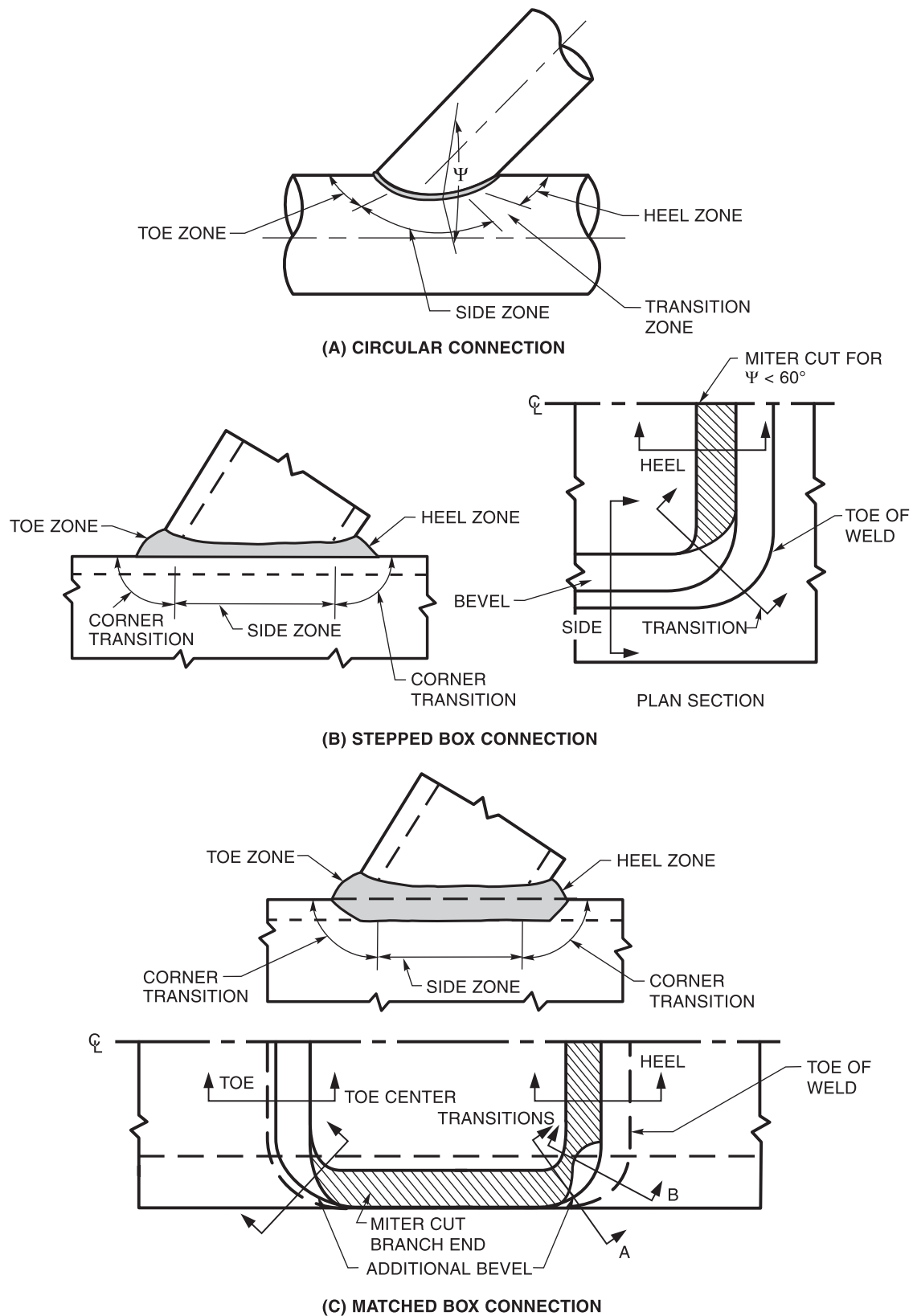
Figure 9.11—Prequalified Joint Details for PJP T-, Y-, and K-Tubular Connections (see 9.10.1)
