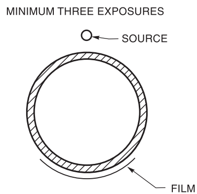
Figure 9.32—Double-Wall Exposure— Single-Wall View (see 9.29.1.2)
