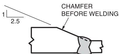
(C) TRANSITION BY CHAMFERING THICKER PART
