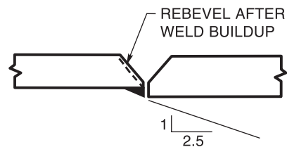
(C) TRANSITION BY TAPER WELD
