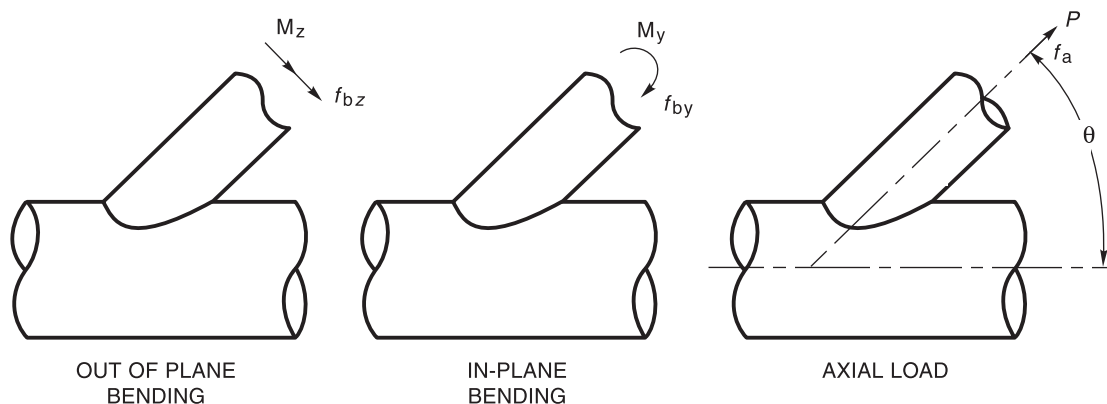
Figure C-9.1—Illustrations of Branch Member Stresses Corresponding to Mode of Loading (see C-9.2.7.2)
