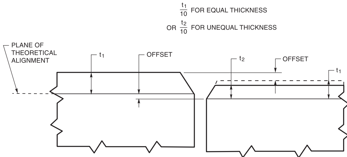
Figure C-5.3—Permissible Offset in Abutting Members (see C-5.21.3)
