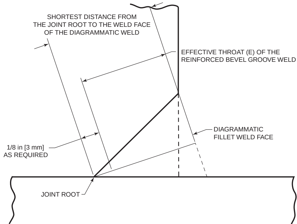
Figure A.4—Bevel Groove Weld with Reinforcing Fillet Weld (see 2.4.2.7)
