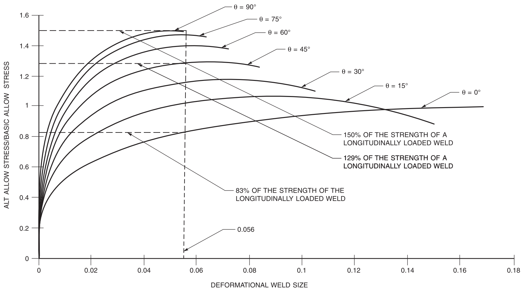
Figure C-2.6—Graphical Solution of the Capacity of an Obliquely Loaded Weld Group (see C-2.6.4.4)
