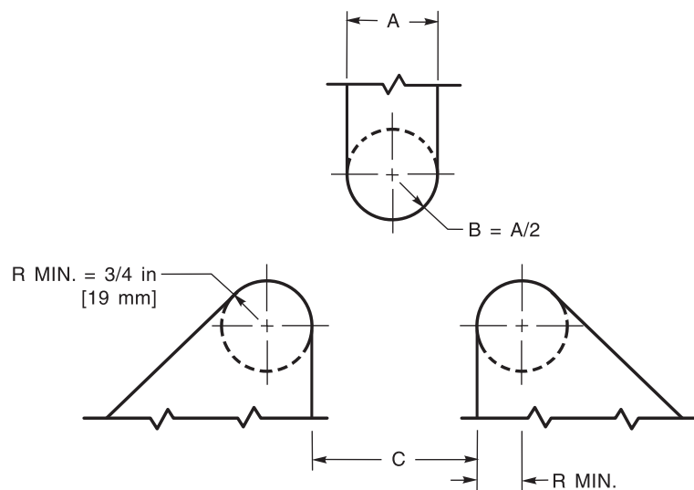
Figure 4.12—Alternative Wraparound Guided Bend Test Jig (see 4.9.3.1)
