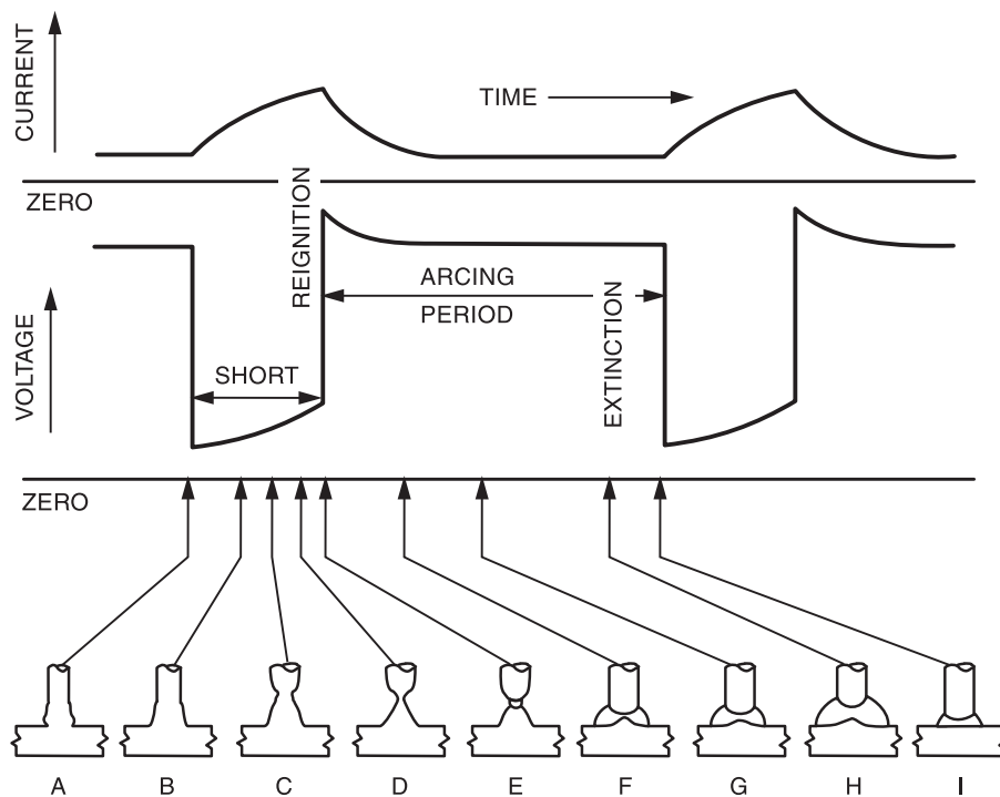
Figure C-3.1—Oscillograms and Sketches of GMAW-S Metal Transfer (see C-3.2.1)
