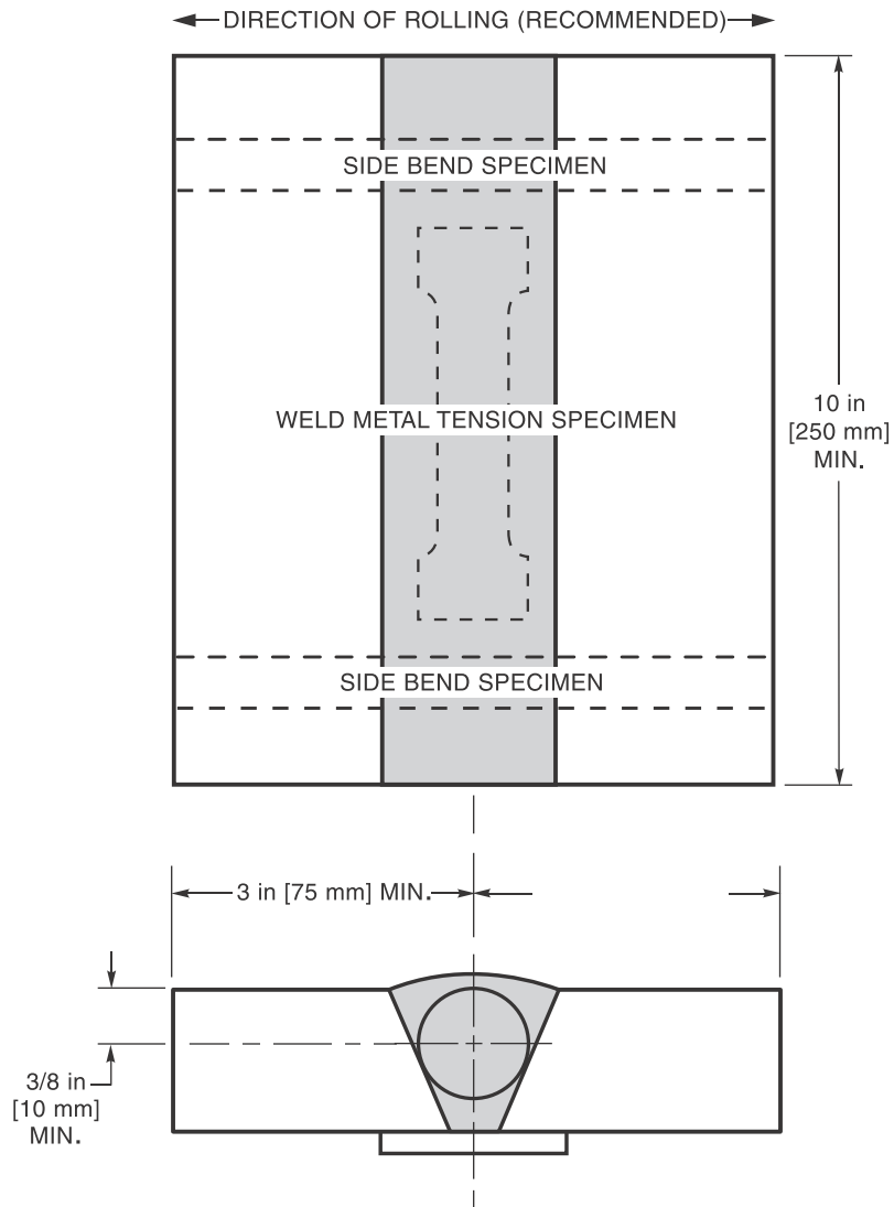
Figure 4.18—Location of Test Specimen on Welded Test Plate 1 in [25 mm] Thick—Consumables Verification for Fillet Weld WPS Qualification (see 4.12.3)
