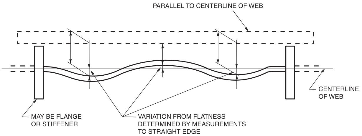
Figure C-5.5—Typical Method to Determine Variations in Girder Web Flatness (see C-5.22.6.1)
