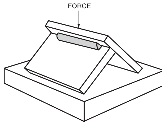
Figure 4.23—Method of Rupturing Specimen—Tack Welder Qualification (see 4.23)
