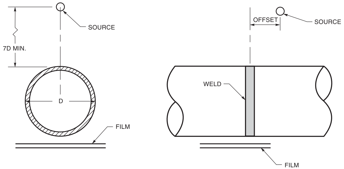
Figure 9.33—Double-Wall Exposure—Double-Wall (Elliptical) View, Minimum Two Exposures (see 9.29.1.3)
