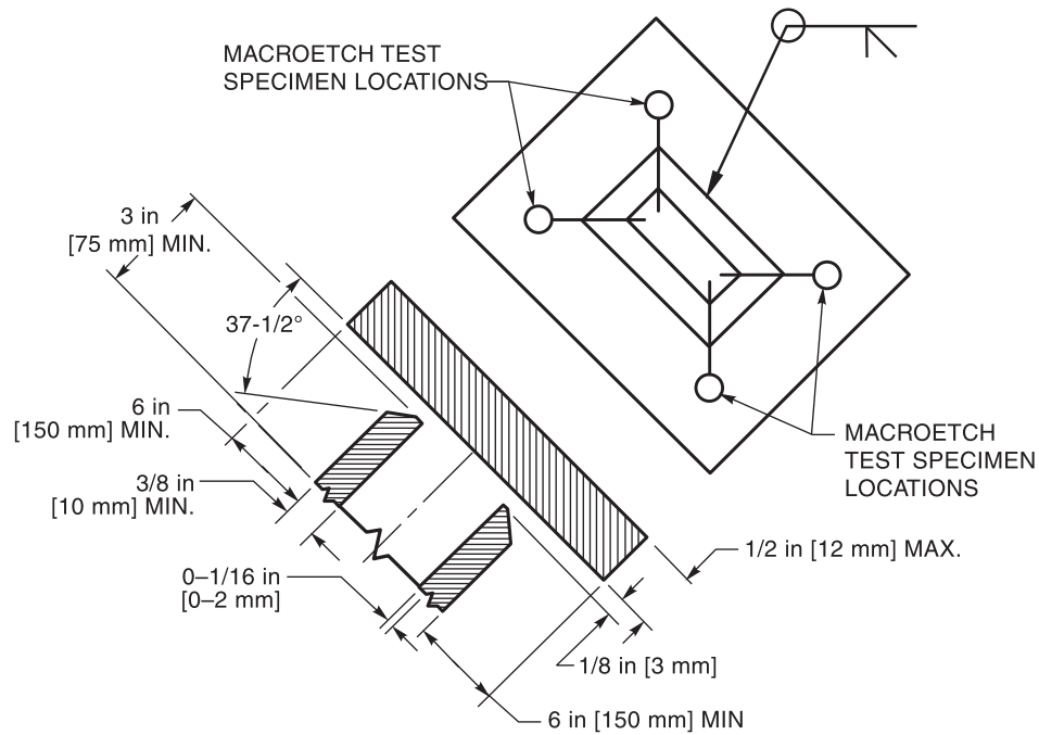
Figure 9.27—Corner Macroetch Test Joint for T-, Y-, and K-Connections without Backing on Box Tubing for CJP Groove Welds—Welder and WPS Qualification (see 9.15.4.1 and 9.19)
