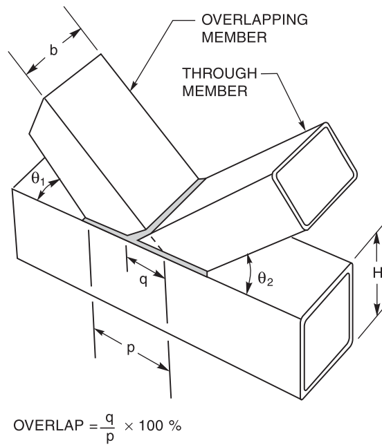
Figure 9.8—Overlapping K-Connections (see 9.6.2.4)
