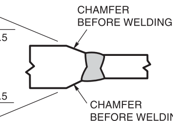
(C) TRANSITION BY CHAMFERING THICKER PART
