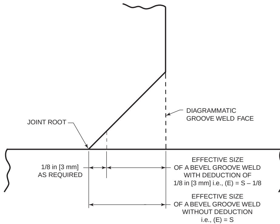
Figure A.2—Unreinforced Bevel Groove Weld
