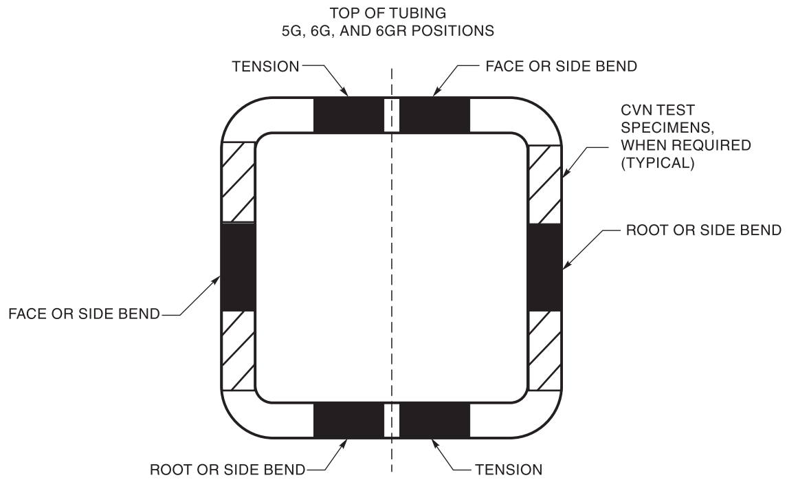
Figure 9.20—Location of Test Specimens for Welded Box Tubing— WPS Qualification (see 9.14)
