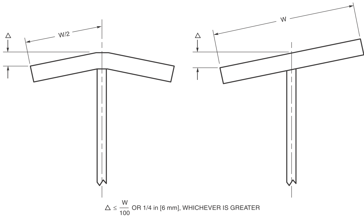
Figure C-5.7—Measurement of Flange Warpage and Tilt (see C-5.22.8)
