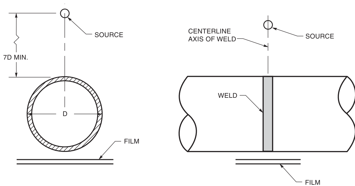
Figure 9.34—Double-Wall Exposure—Double-Wall View, Minimum Three Exposures (see 9.29.1.3)
