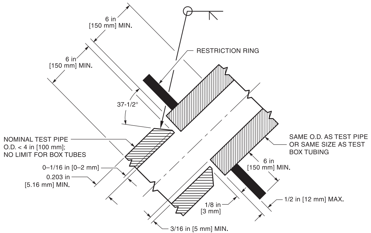
Figure 9.26—Test Joint for T-, Y-, and K-Connections without Backing on Pipe or Box Tubing (<4 in [100 mm] O.D.)—Welder and WPS Qualification (see 9.15.4.1 and 9.19)
