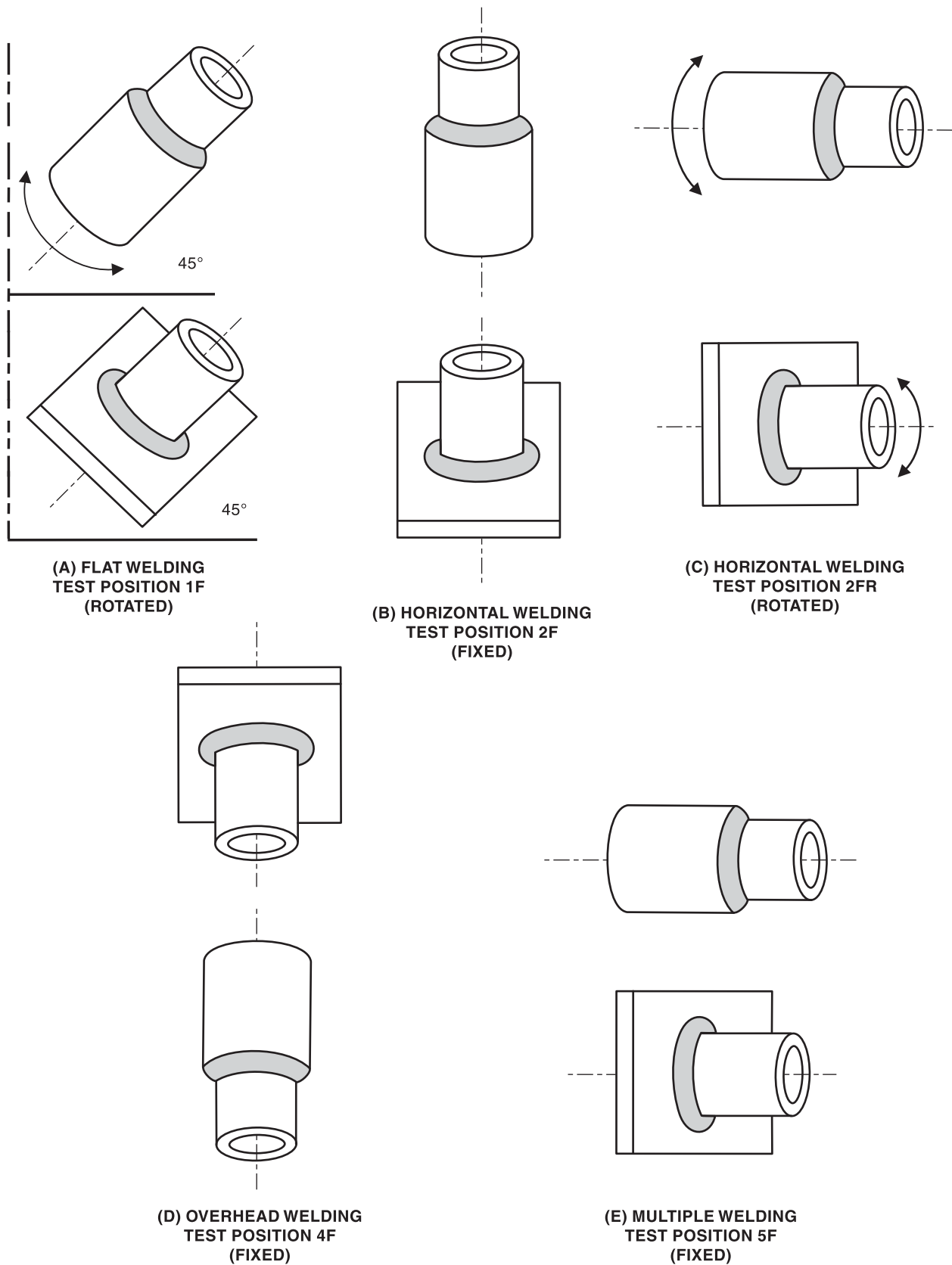
Figure 9.18—Positions of Test Pipes or Tubing for Fillet Welds (see 9.12.1)
