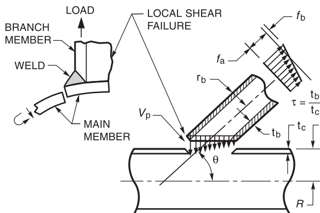
Figure C-9.3—Simplified Concept of Punching Shear (see C-9.6.1.1)
