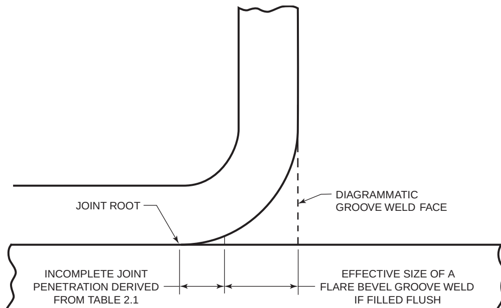
Figure A.5—Unreinforced Flare Bevel Groove Weld
