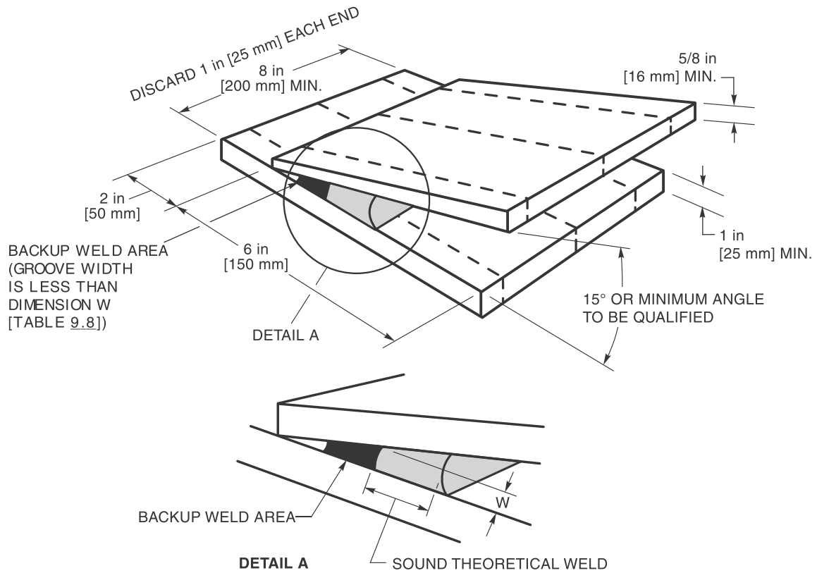
Figure 9.24—Acute Angle Heel Test (Restrains not Shown) (see 9.15.4.2)
