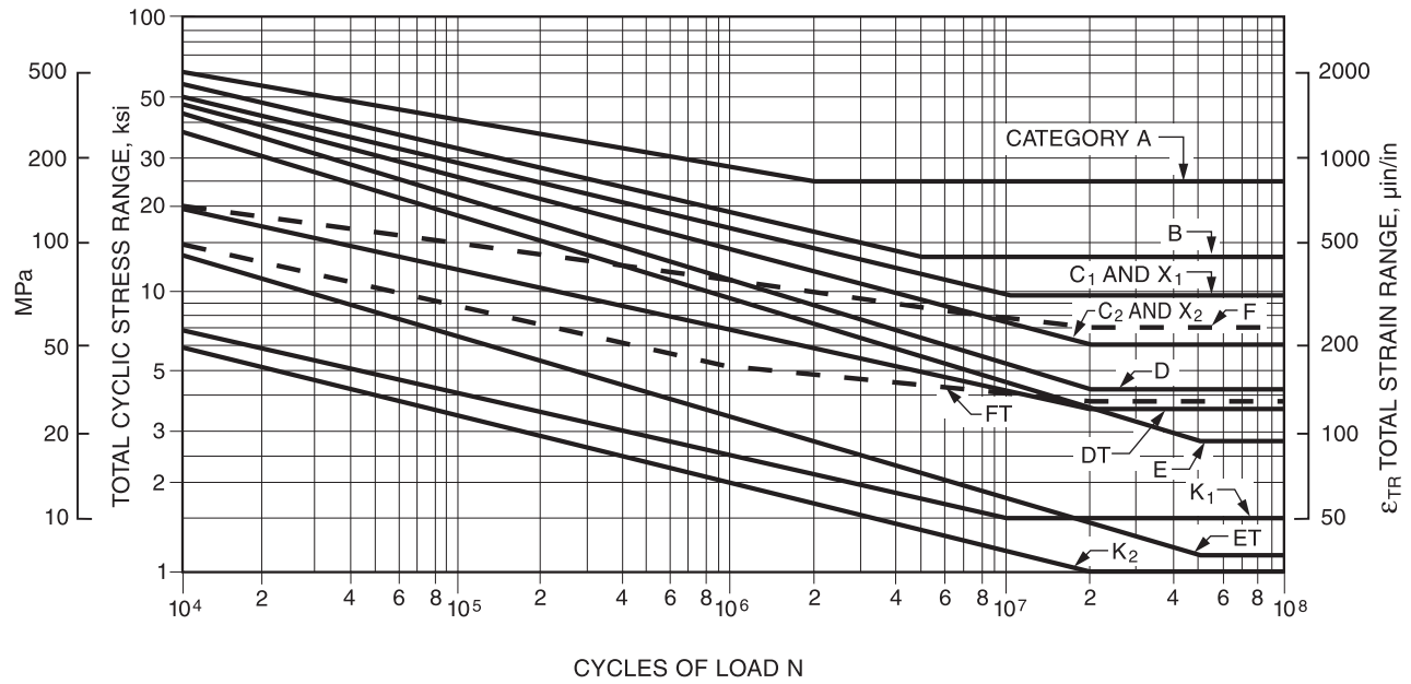
Figure 9.1—Allowable Fatigue Stress and Strain Ranges for Stress Categories (see Table 9.3), Tubular Structures for Atmospheric Service (see 9.2.7.3)
