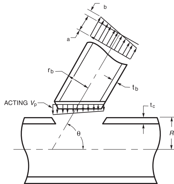
Figure 9.5—Punching Shear Stress (see 9.6.1.1)
