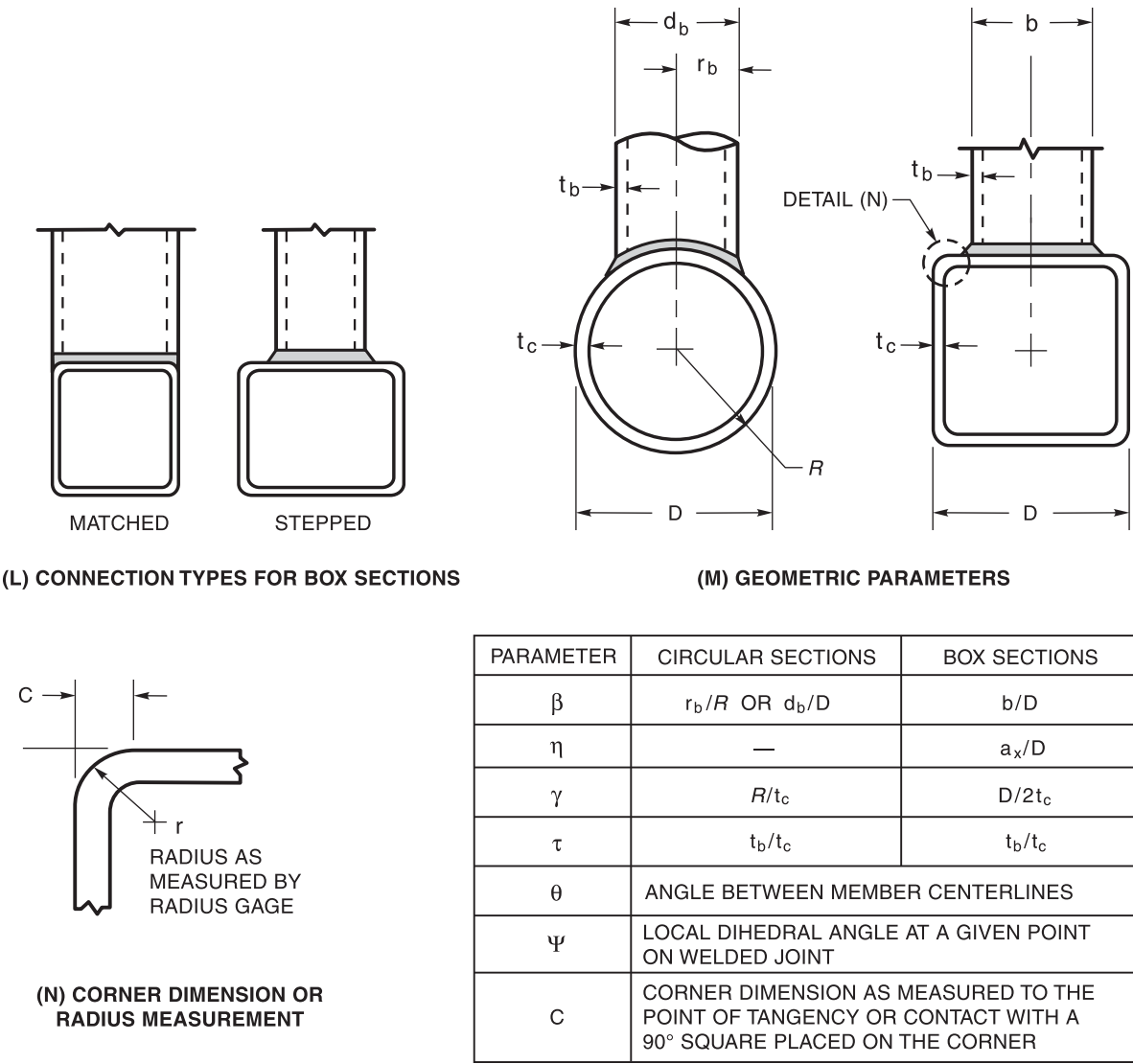
Figure 9.2 (Continued)—Parts of a Tubular Connection (see 9.3)
