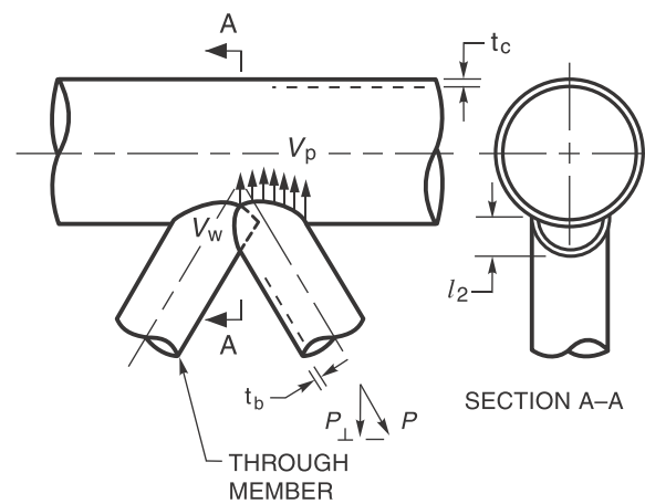
Figure 9.6—Detail of Overlapping Joint (see 9.6.1.6)
