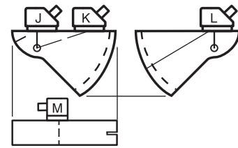
DSC BLOCK
