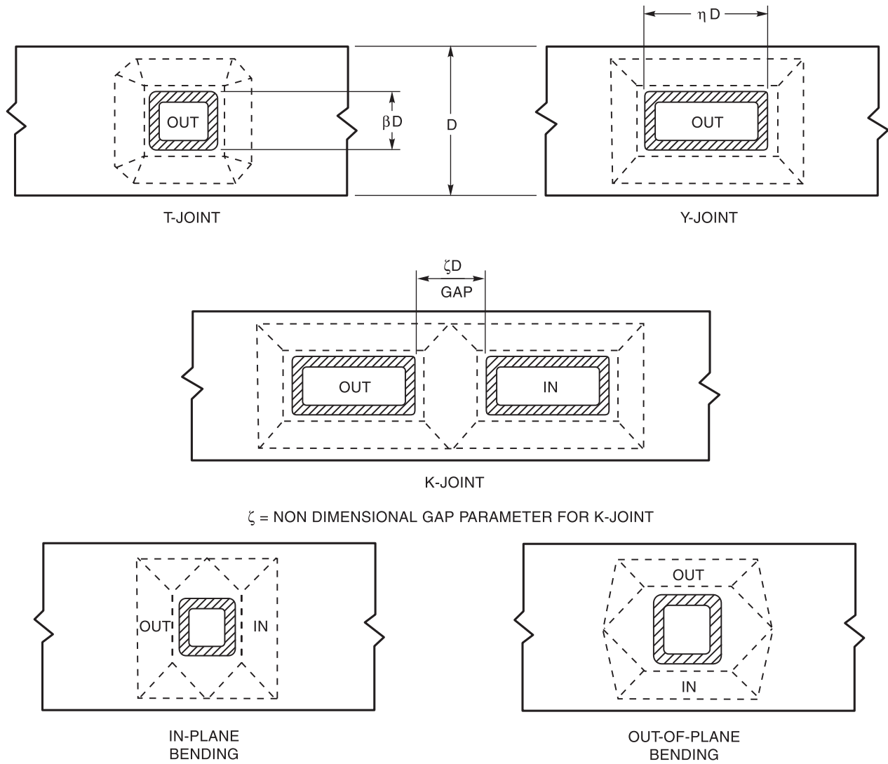
Figure C-9.7—Yield Line Patterns (see C-9.6.2 and C-9.8)
