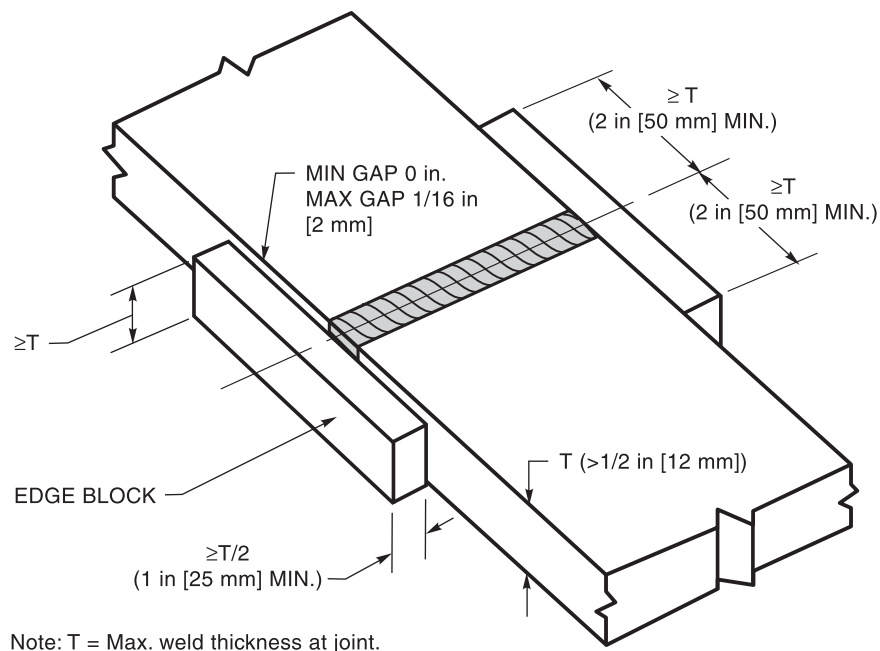
Figure 6.10—RT Edge Blocks (see 6.17.13)
