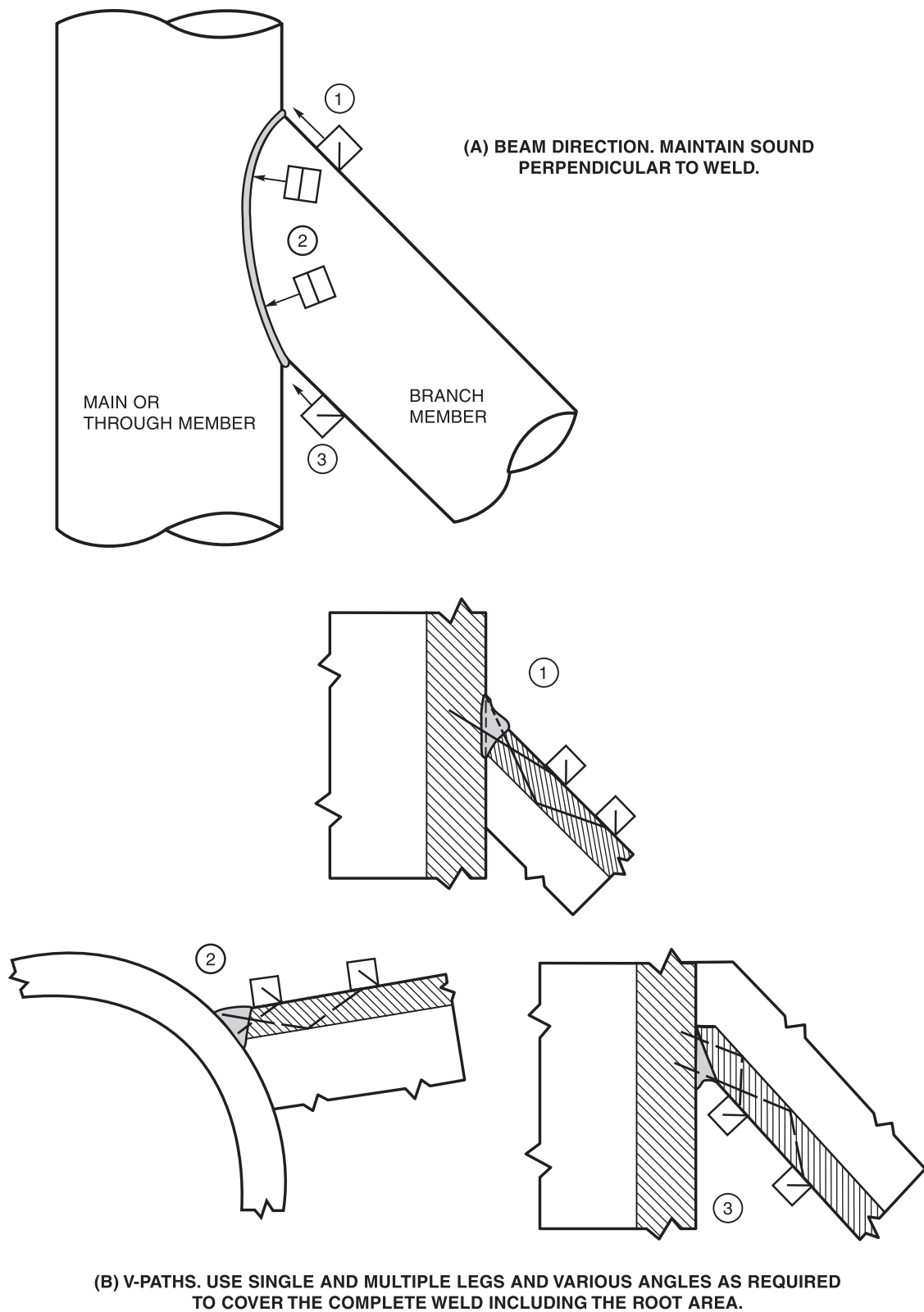
Figure 9.35—Scanning Techniques (see 9.30.5)
