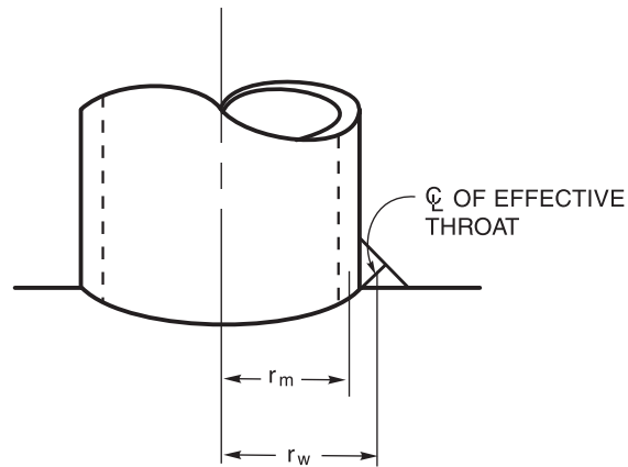
Figure 9.4—Tubular T-, Y-, and K-Connection Fillet Weld Footprint Radius (see 9.5.3)
