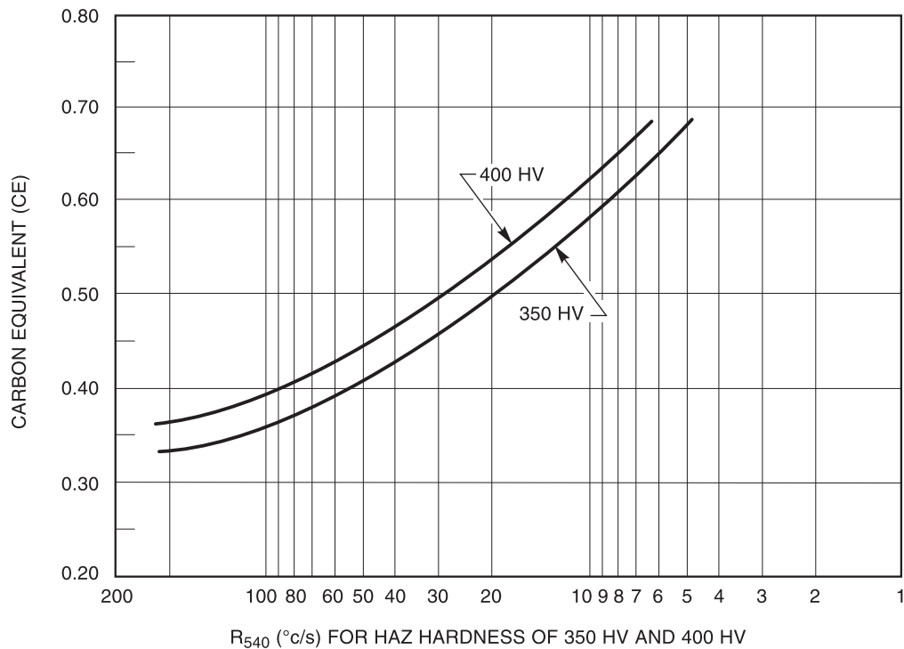
Figure H.2—Critical Cooling Rate for 350 HV and 400 HV (see H3.3)
