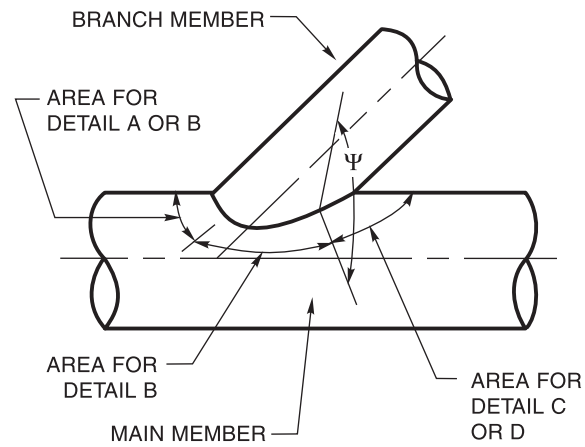
Figure 9.13—Definitions and Detailed Selections for Prequalified CJP T-, Y-, and K-Tubular Connections (see 9.11.2 and Table 9.7)
