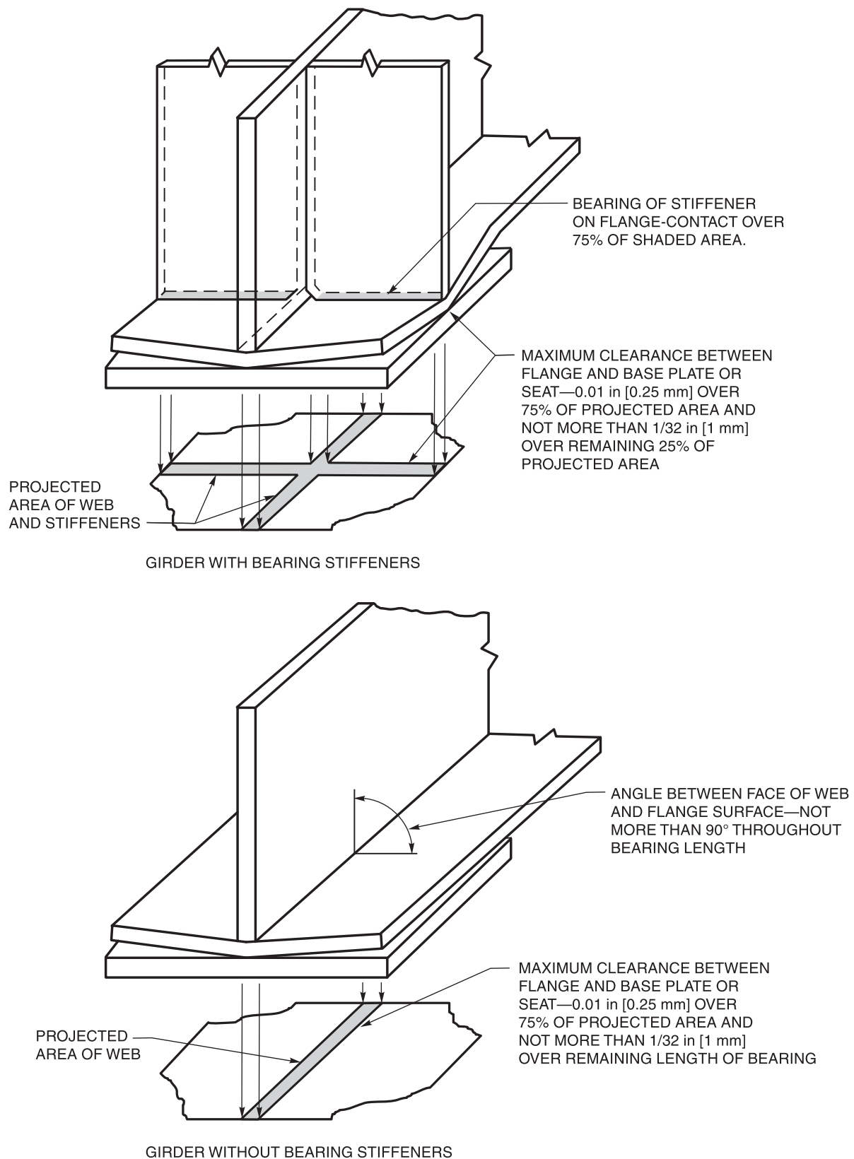
Figure C-5.8—Tolerances at Bearing Points (see C-5.22.10)
