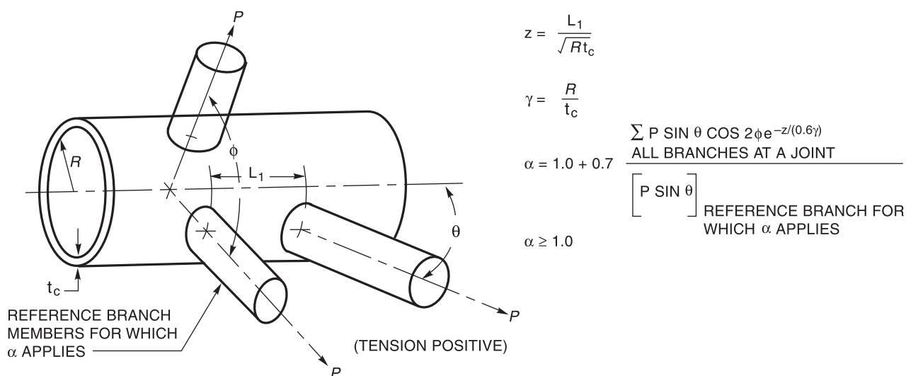
Figure R.1—Definition of Terms for Computed Alpha
