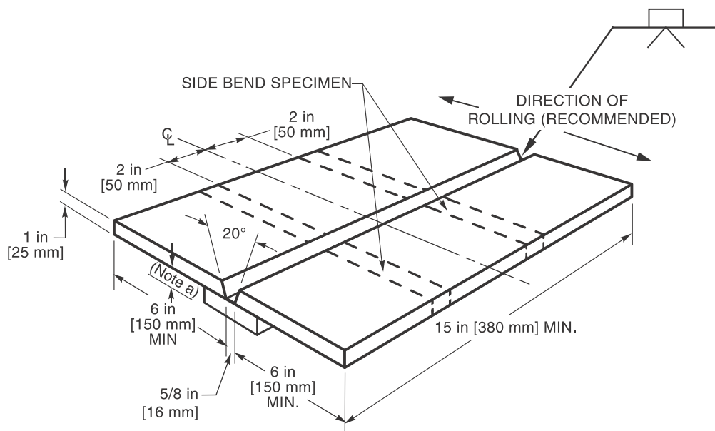
Figure 4.16—Test Plate for Unlimited Thickness—Welder Qualification and Fillet Weld Consumable Verification Tests (see 4.12.3.2 and 4.20.1)
