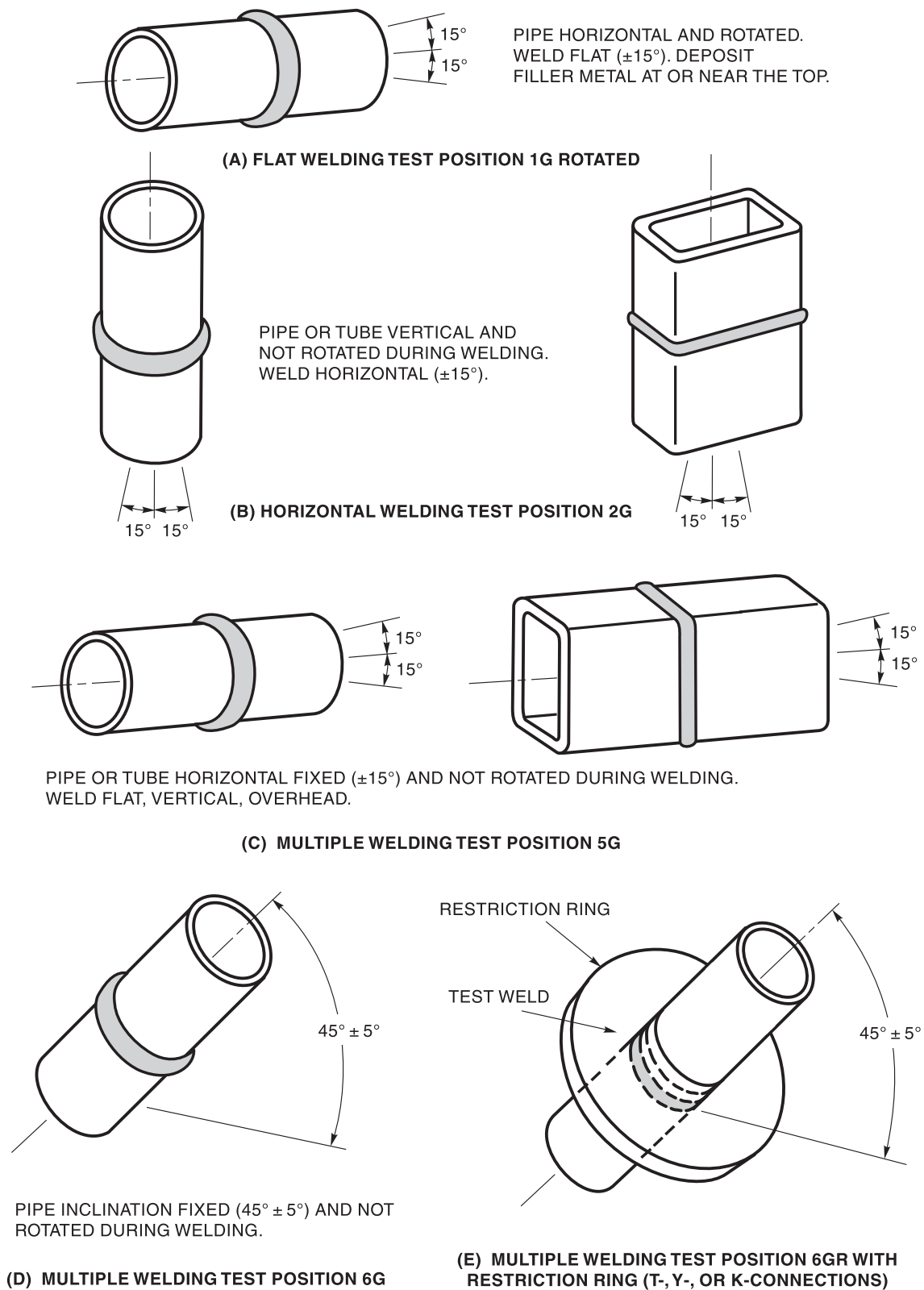
Figure 9.17—Positions of Test Pipe or Tubing for Groove Welds (see 9.12.1)
