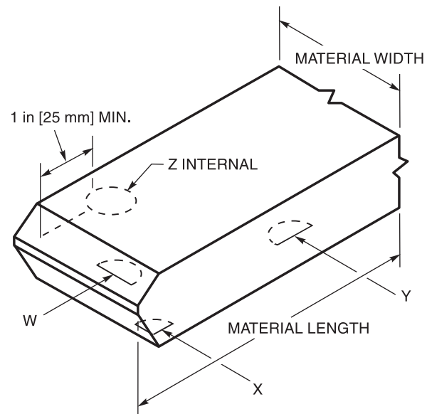
Figure 5.1—Edge Discontinuities in Cut Material (see 5.14.5.1)
