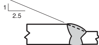
(A) TRANSITION BY SLOPING WELD SURFACE
